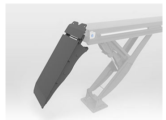
HDSF0713-180H 2 ascending ramps, hanging, 1800 mm
